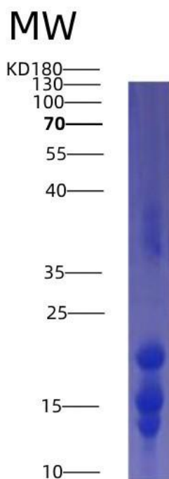
Figure 2. SDS-PAGE
